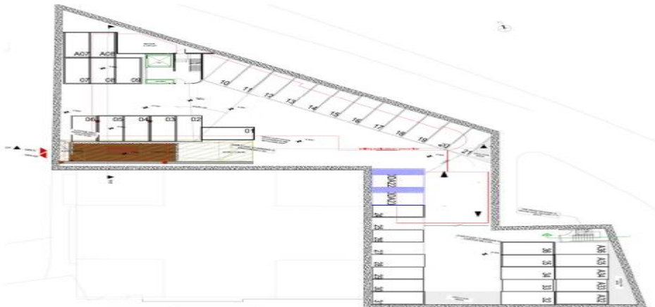
3 - Basement plan
